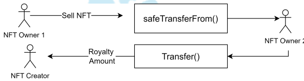
Fig. 6. Consecutive Token Transfers after setting Royalty
